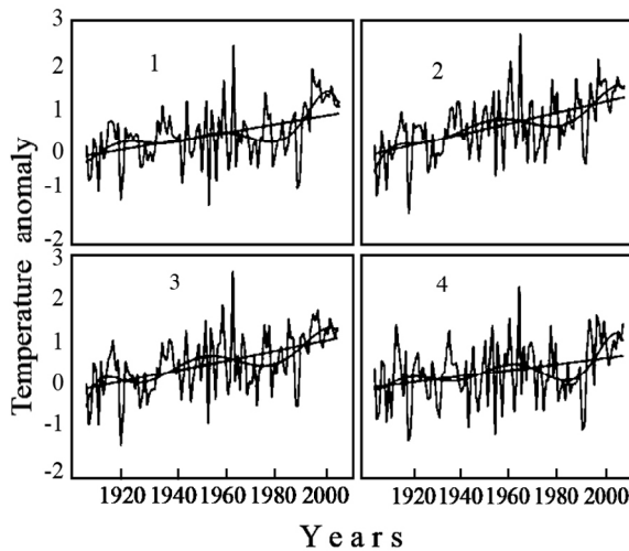
Fig. 2. Changes of temperature anomalies for 4 regions of Georgia (see Fig.1), their linear approximation (linear trend) and 7 th order polynomial approximation (nonlinear trend).
