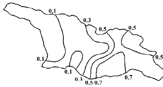
Fig. 3. Temperature field change in Georgia in 1906-2009.
