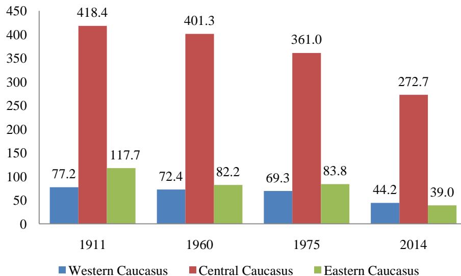
Figure 3. The change in the area (km 2 ) of the Western, Central and Eastern Caucasus glaciers in 1911–1960–1975–2014.
