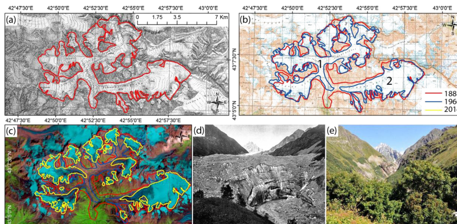
Figure 10. (a) Tviberi glacier, topographical map of 1887; (b) topographical map of 1960; (b1) Tviberi glacier; (b2) Kvitolodi glacier; (c) Landsat L8 imagery; (d) photo of 1884 (M. V. Dechy); (e) photo of 2011 (L. G. Tielidze).
