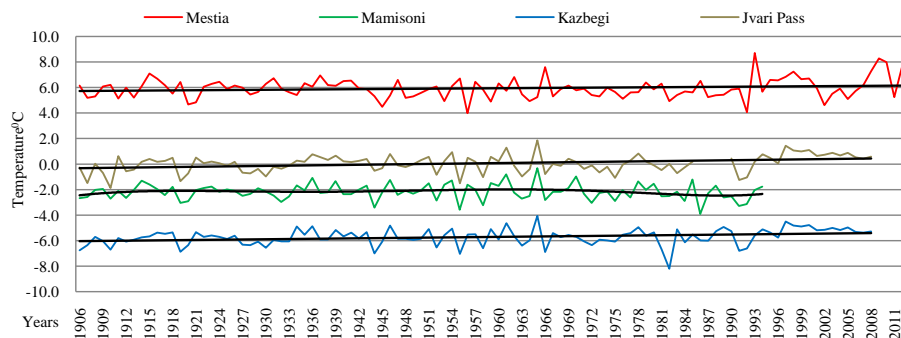
Figure 4. The course of the mean annual air temperatures in the Mestia, Mamisoni, Jvari Pass and Kazbegi meteorological stations over the last one century.
