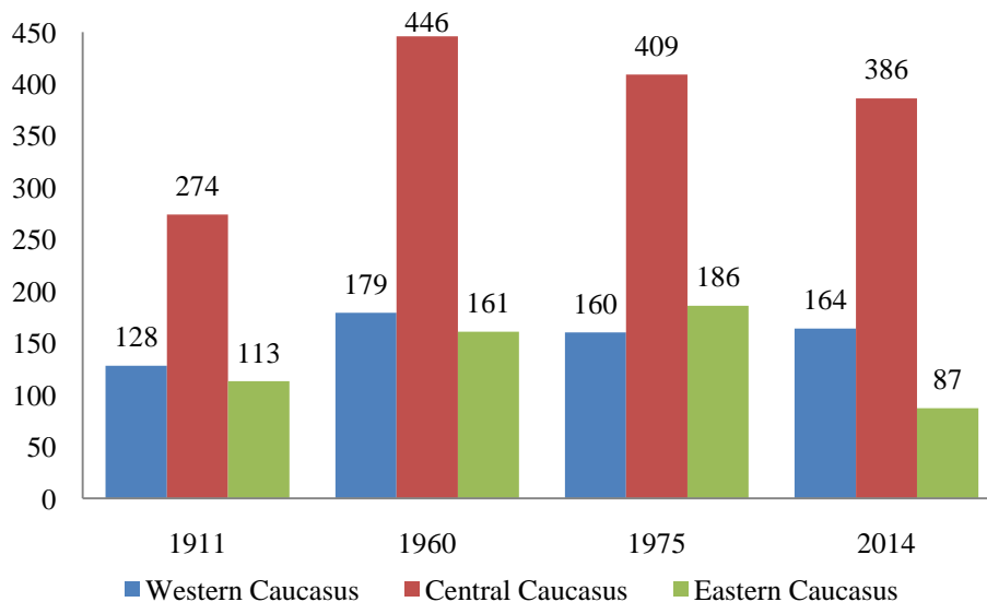
Figure 2. The change in the number of the Western, Central and Eastern Caucasus glaciers in 1911–1960–1975–2014.
