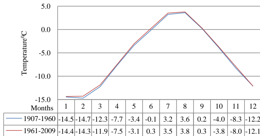
Figure 5. Mean monthly air temperature course of the Kazbegi meteorological station in the years of 1907–1960 and 1961–2009.
