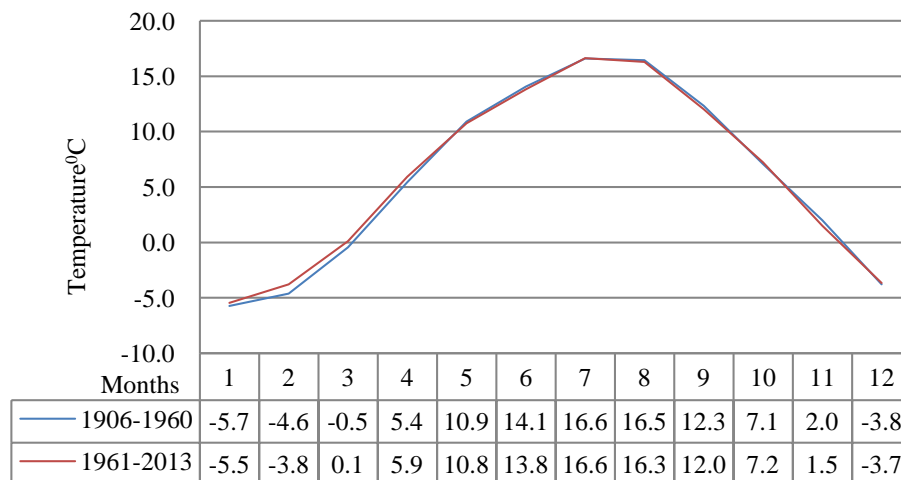
Figure 8. Mean monthly air temperature course of the Mestia meteorological station in the years of 1906–1960 and 1961–2013.
