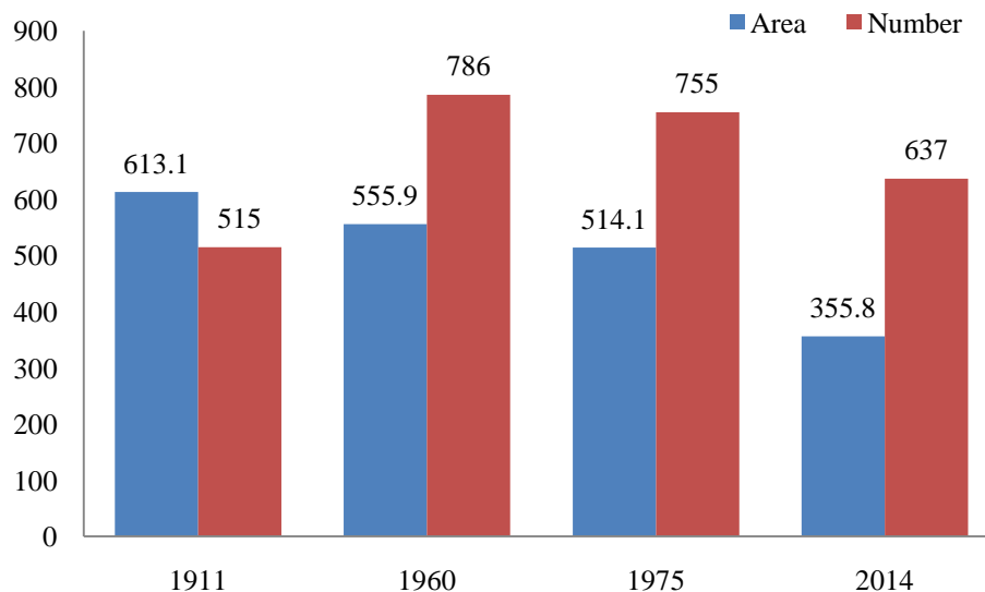
Figure 9. The change in the area (km 2 ) and number of the glaciers of Georgia in 1911–1960–1975–2014.
