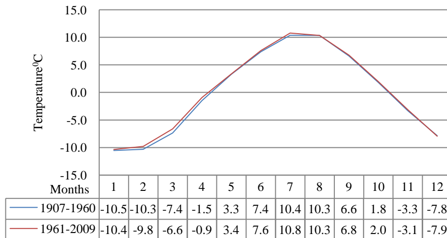
Figure 6. Mean monthly air temperature course of the Jvari Pass meteorological station in the years of 1907–1960 and 1961–2009.
